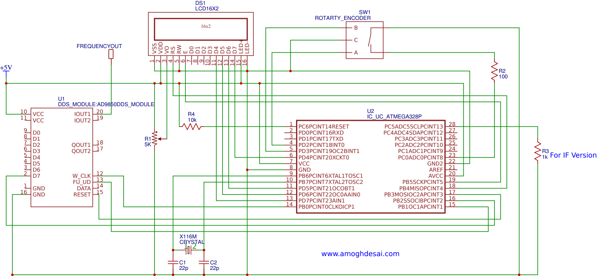
DDS VFO using Arduino and AD9850
